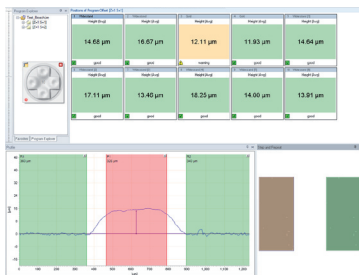
ASCAN user interface with results and data review
